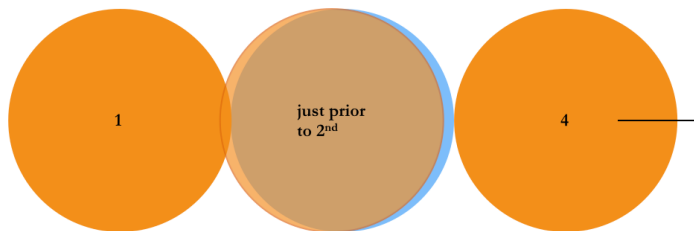
Figure 12.15a: An eclipsing binary, stars having equal diameters.
