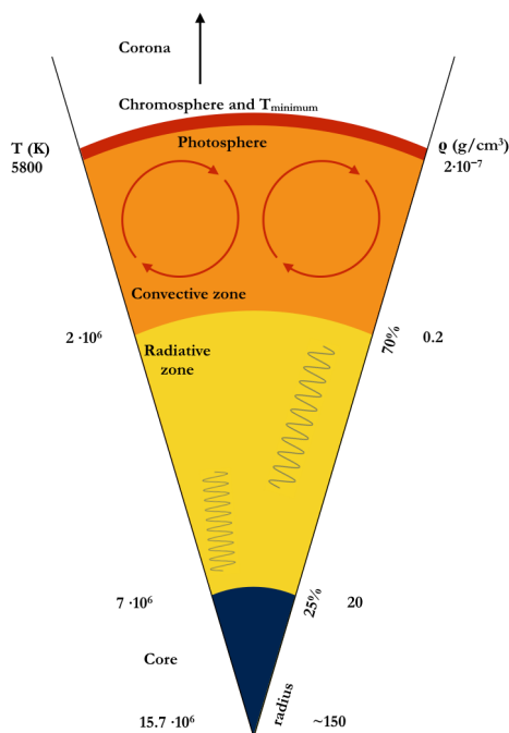
Figure 13.1: Solar structure
