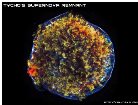
Figure 16.5: Chandra X-ray telescope observation of Tycho's SNR; this image is 9.5 arcminutes across. Red = 1.6 - 2.0 keV; green = 2.2 - 2.6 keV; blue = 4 - 6 keV. Credit: NASA/CXC/SAO.
