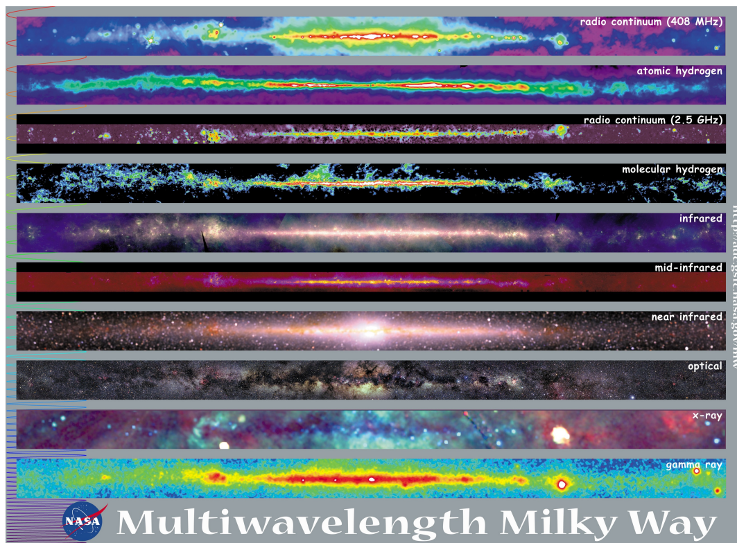
Figure 17.18; http://mwmw.gsfc.nasa.gov/mwpics/mwmw_8x10.jpg
