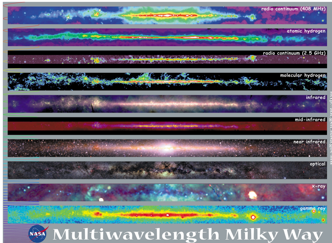
Figure 17.18; http://mwmw.gsfc.nasa.gov/mwpics/mwmw_8x10.jpg
