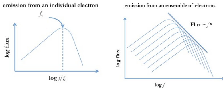
Figure 17.29: synchrotron emission
