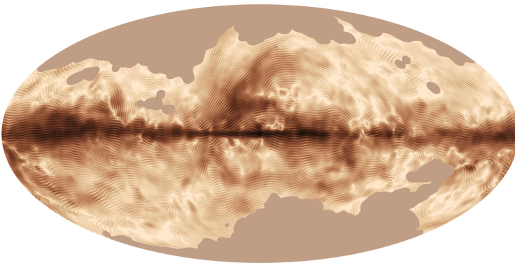
Figure 17.28: Milky Way magnetic field. Credit: ESA and the Planck Collaboration
