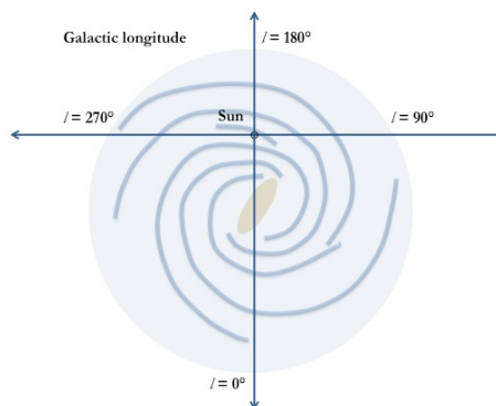
Figure 17.9: galactic coordinates; a) side view, b) top view.
