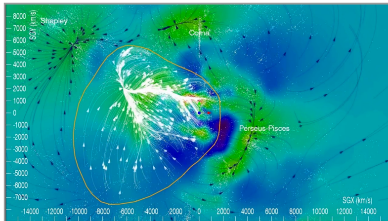
Figure 18.49: Laniakea Supercluster
