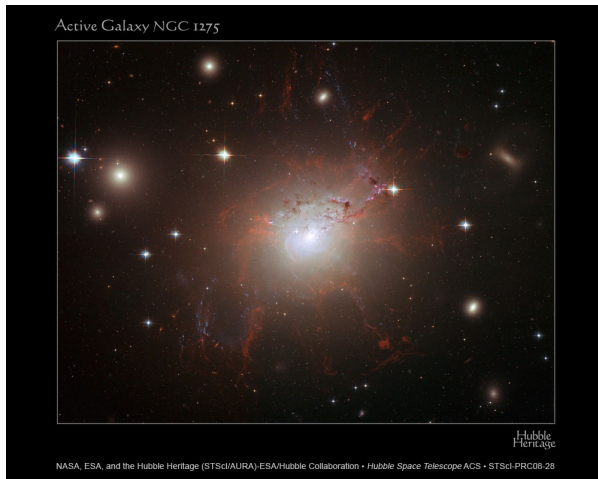
Figure 18.31a http://hubblesite.org/newscenter/archive/releases/2008/28/image/a/
