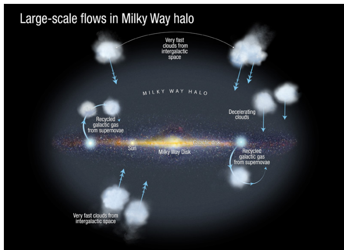
Figure 18.17
