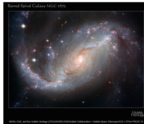
Figure 18.3: NGC 1672
