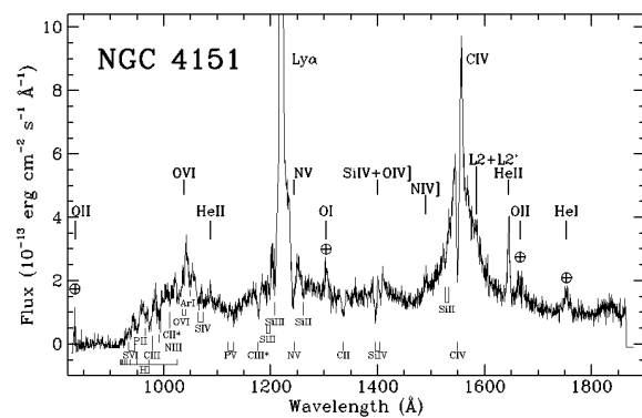
Figure 18.30: NGC 4151 spectrum
