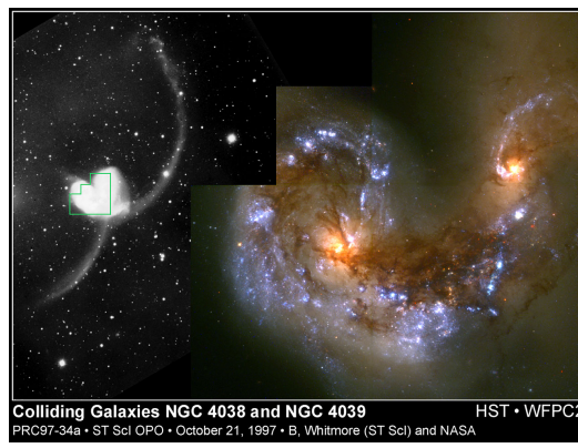
Figure 18.45
