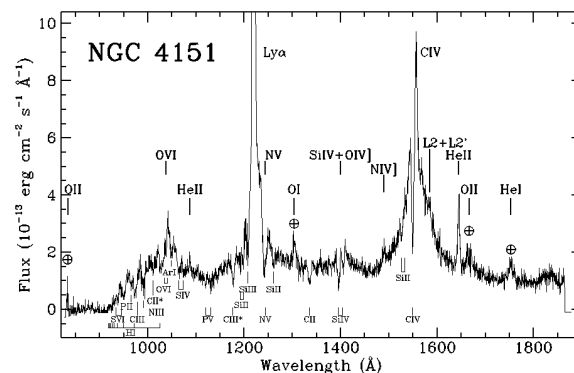
Figure 18.30: NGC 4151 spectrum
