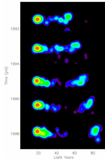
Figure 18.43 a: example of apparent superluminal motion; b: radio image of 3C 279; image courtesy of NRAO/AUI; http://images.nrao.edu/387
