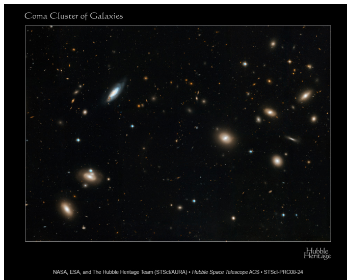
Figure 18.16: Coma cluster
