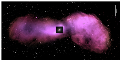
Figure 18.32: Centaurus A; credit: ESO/WFI (Optical); MPIfR/ESO/APEX/A. Weiss et al. (Submillimetre); NASA/CXC/CfA/R. Kraft et al. (X-ray) http://www.eso.org/public/images/eso0903a/
