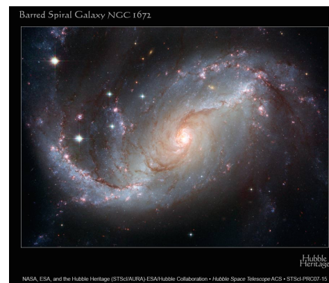
Figure 18.3: NGC 1672
