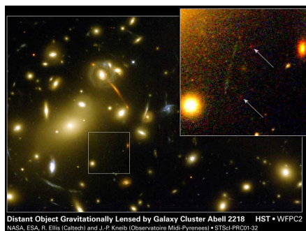
Figure 19.6: Abell 2218; observations by HST and the 10-m Keck telescopes in Hawaii.
