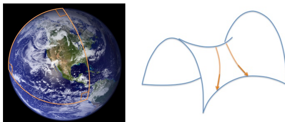
Figure 19.1: a) positively (left) and b) negatively curved (center) two-dimensional surface
