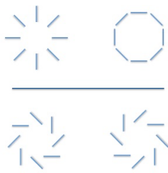
Figure 19.23: E-mode (top two) and B-mode (bottom two) polarization patterns.
