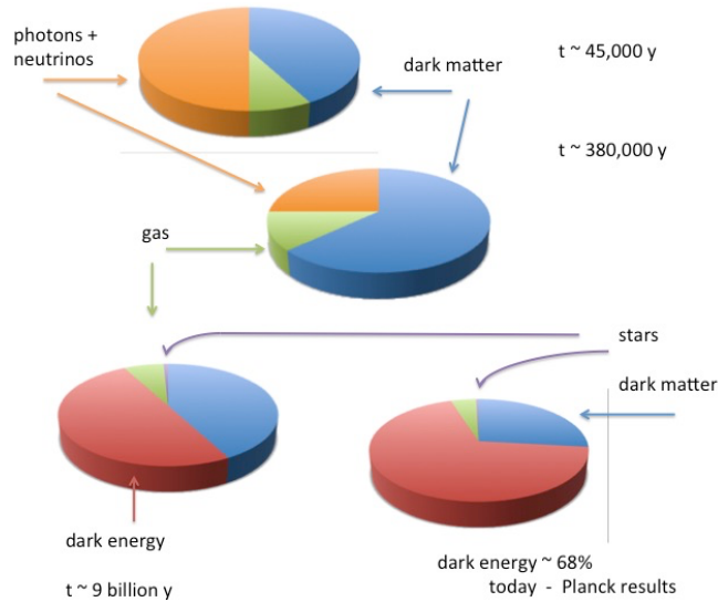
Figure 19.13: Evolution of the relative contributions to the energy density of the universe with time.
