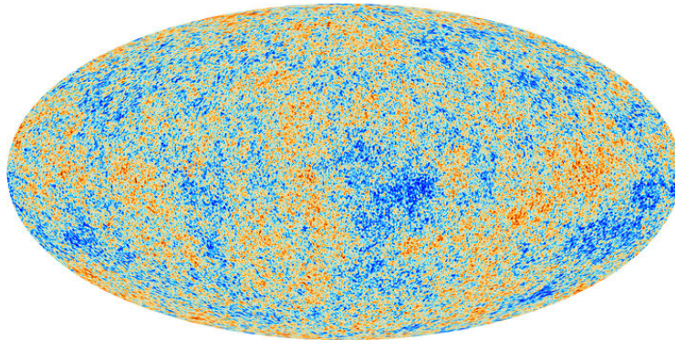
Figure 19.11: Anisotropies in the CMB; credit: ESA and the Planck Collaboration
