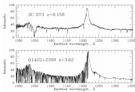
Figure 19.18: quasar spectra from Bill Keel's set of AGN slides. http://www.astr.ua.edu/keel/agn/forest.html
