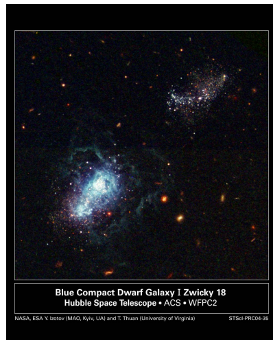
Figure 19.21: low-metallicity galaxy; http://hubblesite.org/image/1621/news_release/2004-35
