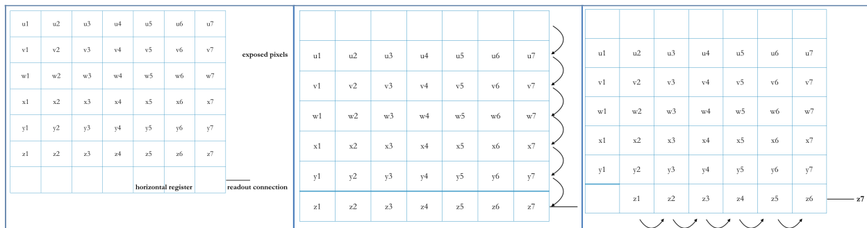
Figure 20.22: CCD readout
