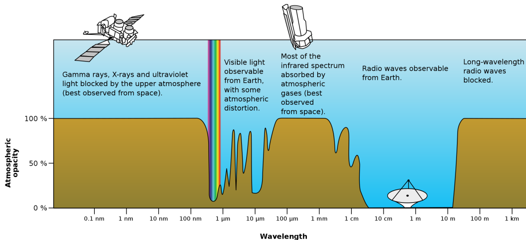
Figure 20.2: Earth's atmospheric opacity as a function of wavelength. Credit: NASA
