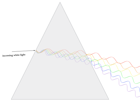
Figure 20.4: refraction
