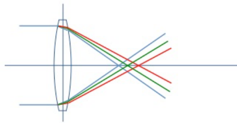
Figure 20.5: chromatic aberration
