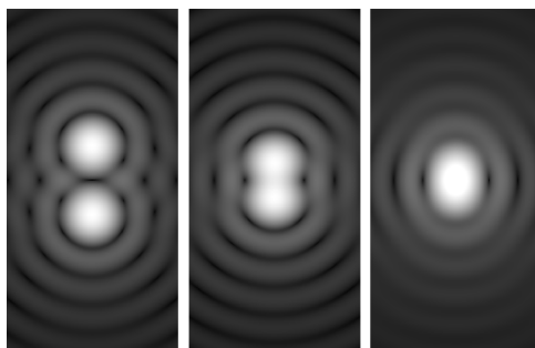
Figure 20.14: Resolution
