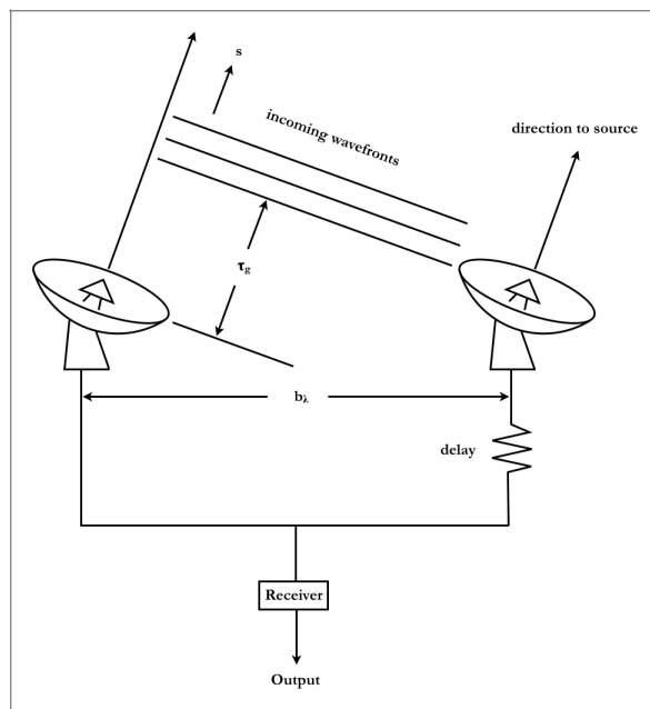
Figure 20.25: Incoming wavefront and the two-element interferometer.
