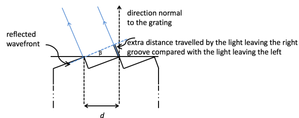
Figure 20.20: Diffraction geometry, reflected light
