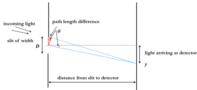
Figure 20.15: Single-slit diffraction
