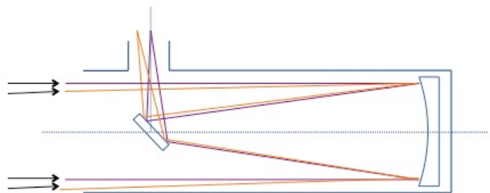
Figure 20.9b): Newtonian reflector light path
