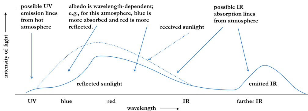
Figure 4.74: Planetary spectrum
