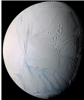
Figure 4.43: Enceladus. Credit: NASA / JPL / Space Science Institute; Cassini spacecraft
