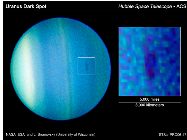
Figure 4.22: Uranus' dark spot http://hubblesite.org/newscenter/archive/releases/2006/47/image/a/
