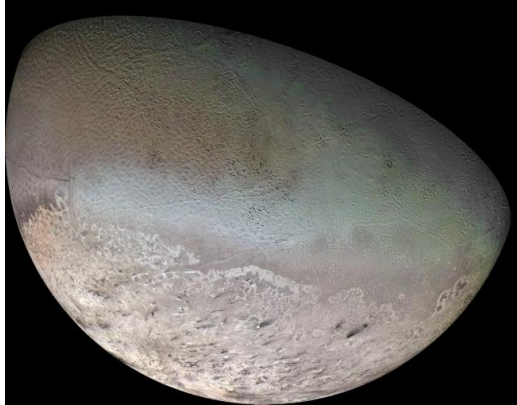
Figure 4.37: Triton. Credit: NASA / JPL / USGS; Voyager 2 http://photojournal.jpl.nasa.gov/catalog/PIA00317
