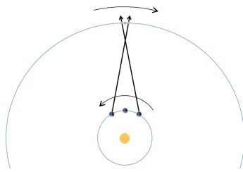
Figure 4.52: Retrograde motion of an outer planet.
