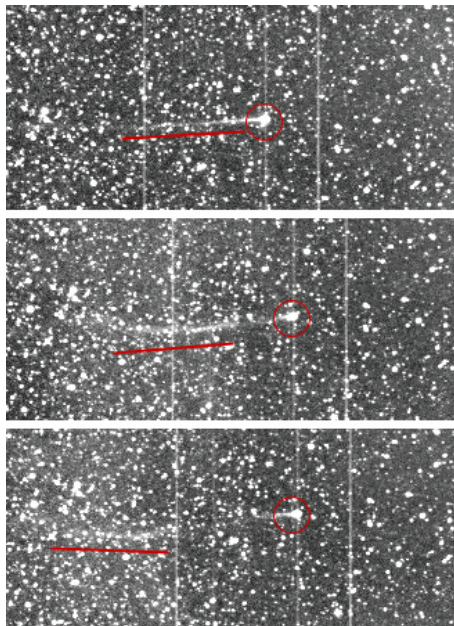
Figure 4.64: Comet Encke and tail disconnection event.
