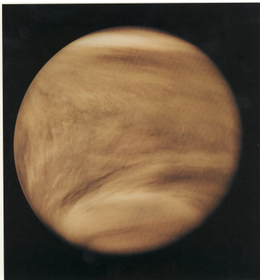
Figure 4.6a: Pioneer Venus
