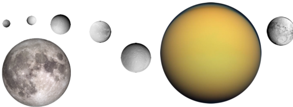
Figure 4.41: Medium-sized moons of Saturn (plus our Moon &amp; Titan)
