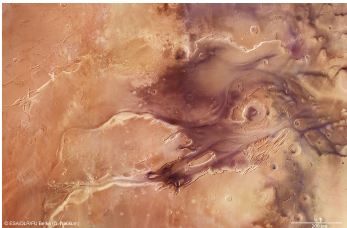
Figure 4.11 a: Kasei Valles Image credit: ESA/DLR/FU Berlin (CC BY-SA); Mars Express http://sci.esa.int/mars-express/55576-kasei-valles-mosaic/
