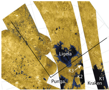
Figure 4.35: Titan.
