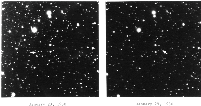
Figure 4.53. Lowell Observatory https://en.wikipedia.org/wiki/Pluto#/media/File:Pluto_discovery_plates.png
