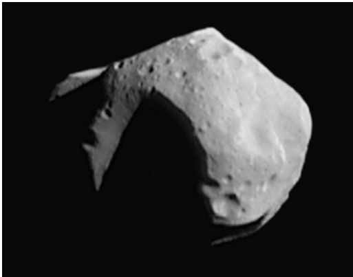
Figure 4.13: 253 Mathilde.
