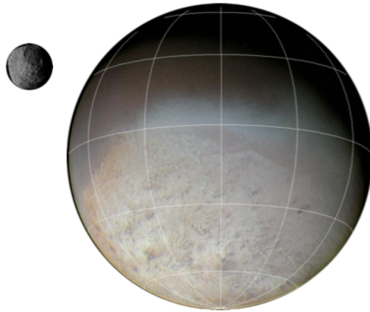
Figure 4.51: Proteus (left) Credit:
