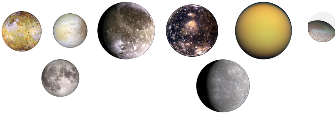
Figure 4.23: Major moons
