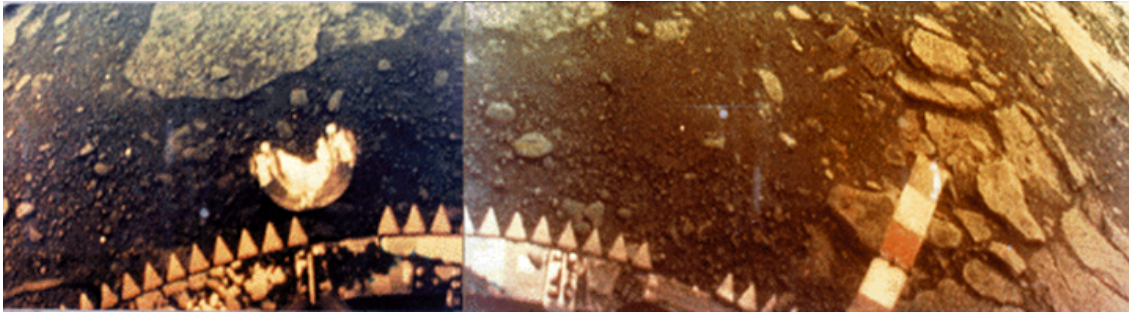
Figure 4.5: Venus, Venera 13
