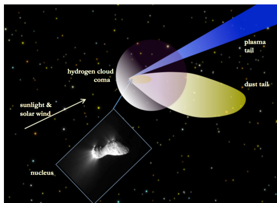
Figure 4.63: Anatomy of a comet
