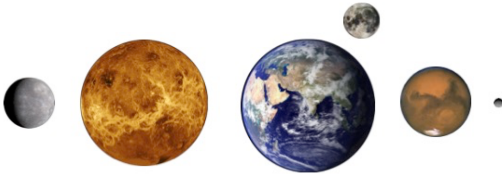
Figure 4.2: Rocky planets
