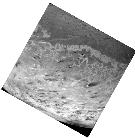
Figure 4.38: Triton Credit: NASA / JPL; Voyager 2 http://photojournal.jpl.nasa.gov/catalog/PIA00059
