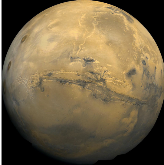
Figure 4.9: Mars. Credit: NASA / Viking Project; USGS
