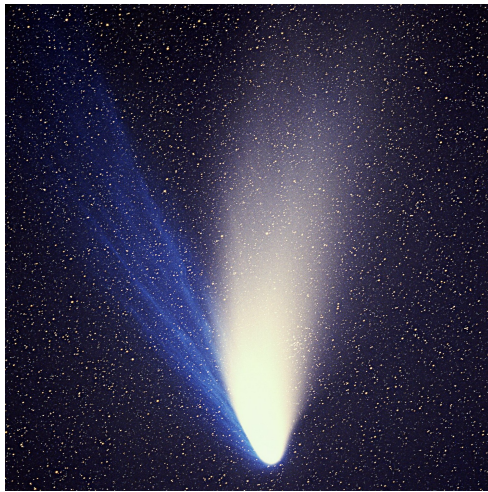
Figure 4.59: Comet Hale-Bopp.
