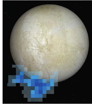
Figure 4.27: Europa's plumes. Credit: NASA/ESA/L. Roth/SWRI/University of Cologne http://www.nasa.gov/content/goddard/water-vapor-over-europa
