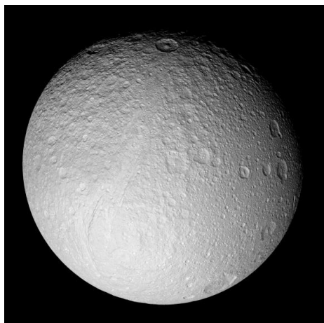
Figure 4.44: Tethys
