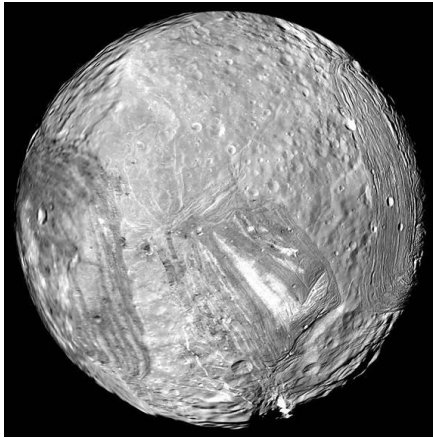
Figure 4.50: Miranda
