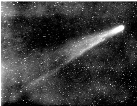
Figure 4.66: Yerkes Observatory photo of Halley's Comet, 1910
