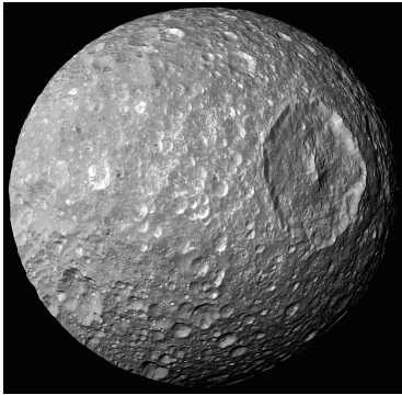
Figure 4.42: Mimas
