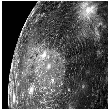
Figure 4.32: Callisto and Valhalla impact basin. Credit: NASA / JPL; Voyager 1 http://photojournal.jpl.nasa.gov/catalog/PIA02277
