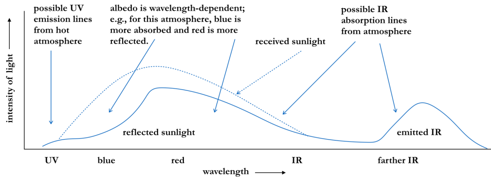
Figure 4.74: Planetary spectrum
