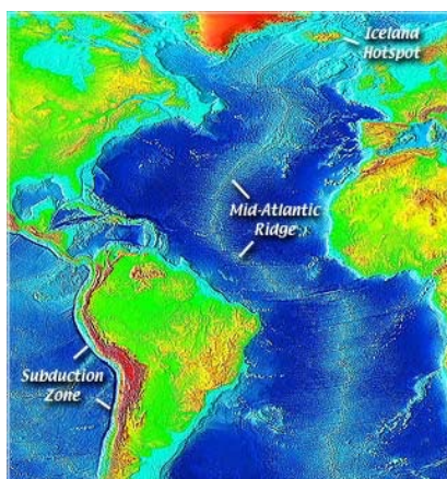
Figure 5.10: Mid-Atlantic Ridge
