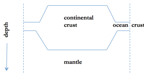
Figure 5.3: Isostatic compensation
