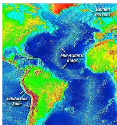
Figure 5.10: Mid-Atlantic Ridge
