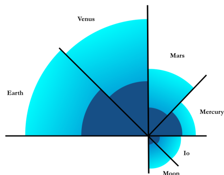
Figure 5.17: Core sizes for rocky objects.
