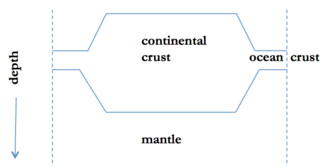
Figure 5.3: Isostatic compensation
