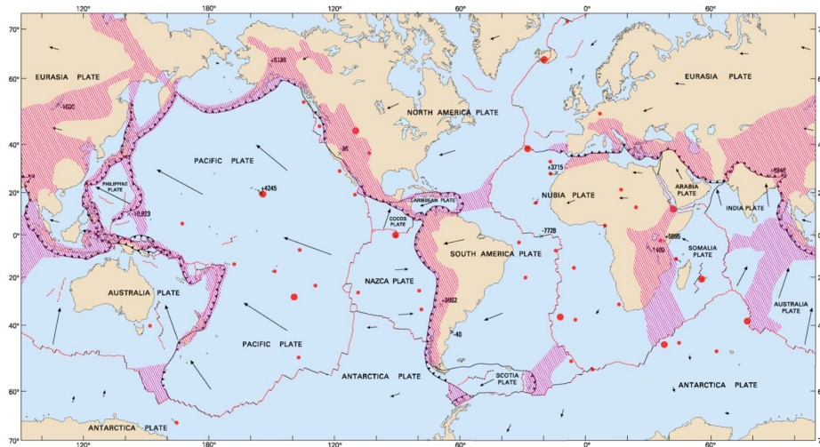
Figure 5.11: Tectonic plates
