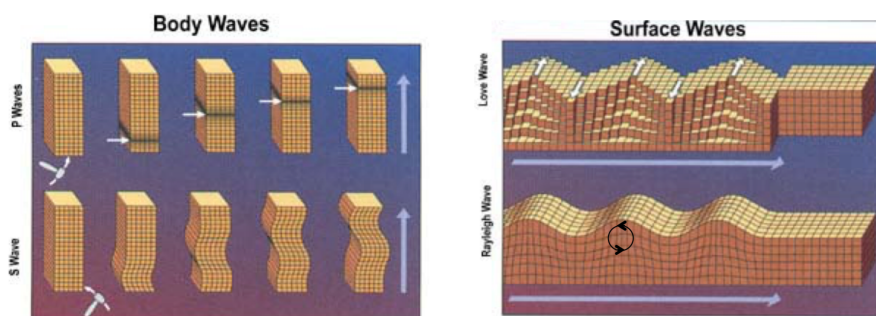
Figure 5.4: Seismic waves
