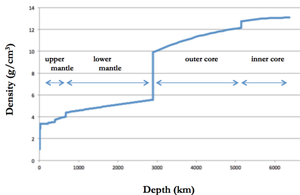
Figure 5.16: Preliminary Reference Earth Model
