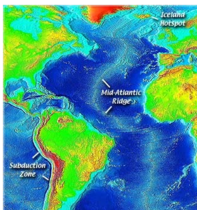
Figure 5.10: Mid-Atlantic Ridge
