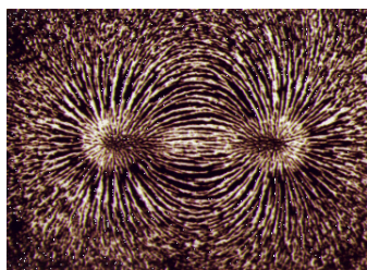
Figure 5.14: Dipole magnetic field
