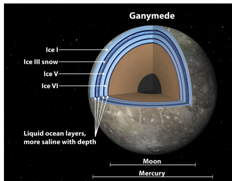
Figure 5.18: Ganymede interior model
