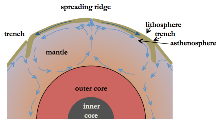
Figure 5.8: Plate tectonics
