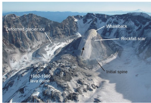
Figure 6.33: Mount St. Helens crater, Feb. 2005.
