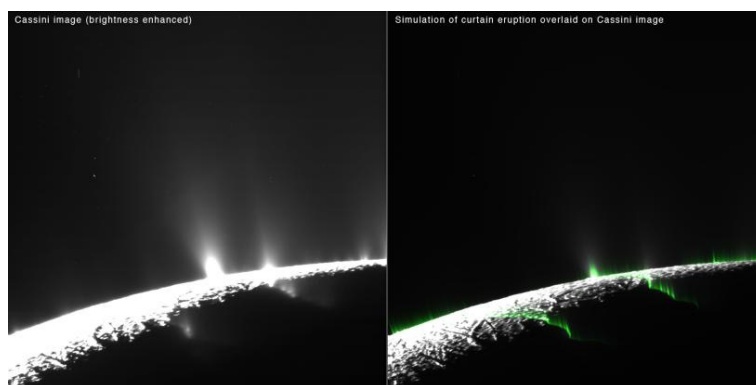
Figure 6.42: Curtain eruptions on Enceladus NASA / Cassini spacecraft http://photojournal.jpl.nasa.gov/catalog/PIA19061
