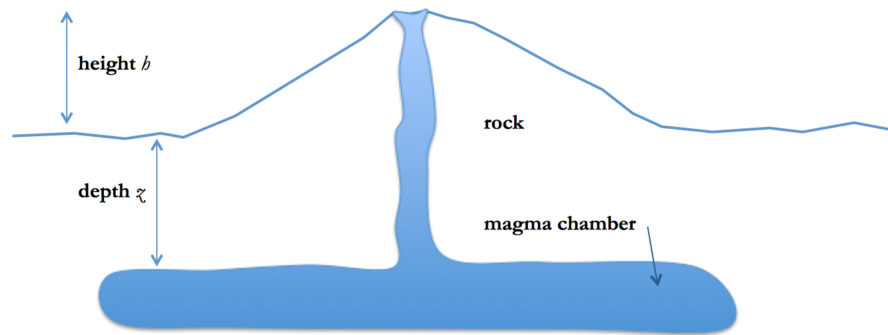
Figure 6.34: Volcano height
