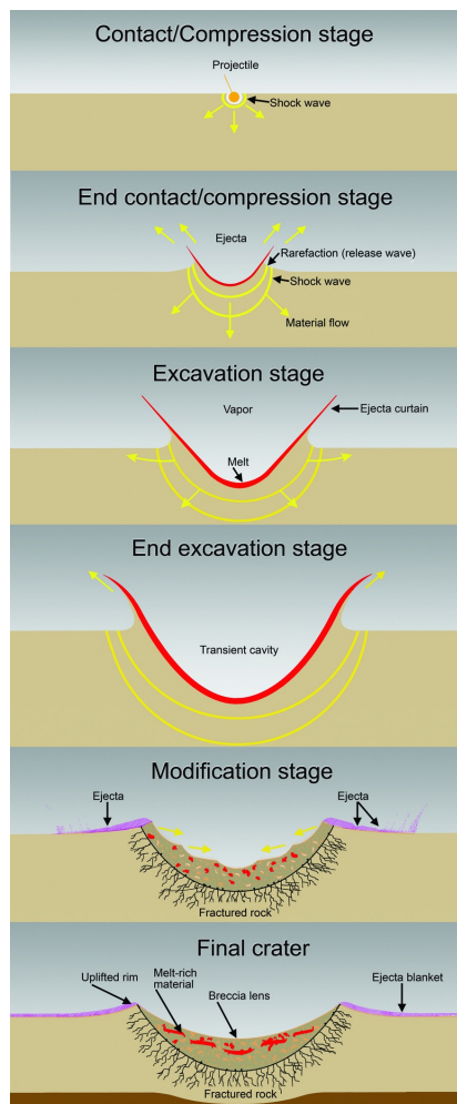
Figure 7.7: Formation of simple (left) and complex (below) craters.
