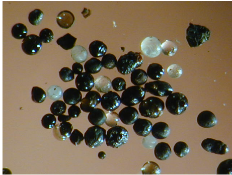
Figure 7.26: Cosmic spherules.
