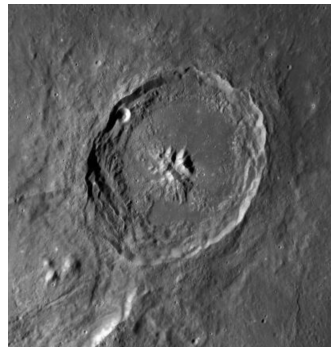
Figure 7.8: Lunar craters a) Rosse, b) Theophilus, c) multi-ring basin Mare Orientale
