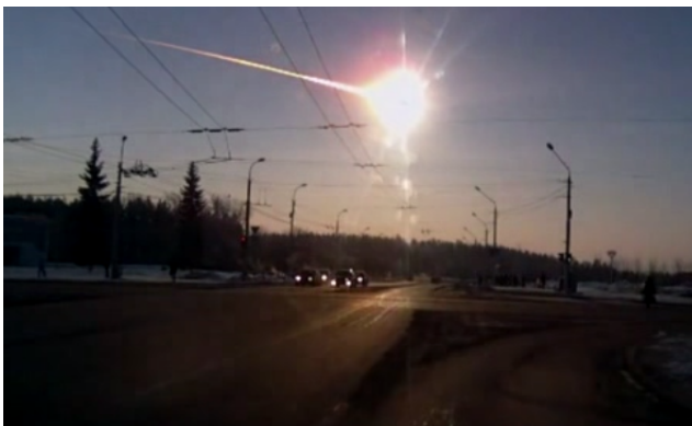
Figure 7.40: Chelyabinsk event.
