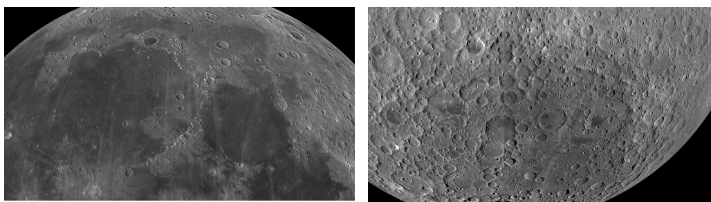
Figure 7.15: a) Mare Imbrium and Mare Serenitatis on the near side (left) and b) the South Pole - Aitken basin on the far (right) side of the Moon. Credit: NASA / GSFC / Arizona State University. Lunar Reconnaissance Orbiter mosaics. http://roc.sese.asu.edu/posts/298
