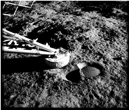
Figure 7.3: Lunar regolith
