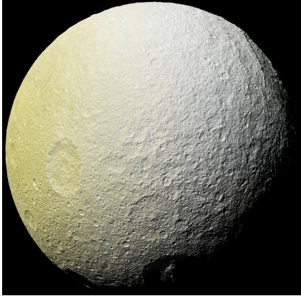
Figure 7.17: Tethys
