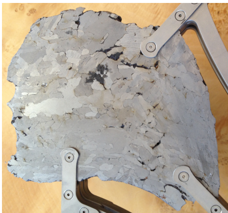
Figure 7.30: The interior of the Campo del Cielo iron fragment shown above.
