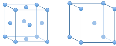
Figure 7.28: Face-centered cubic (far left) and body-centered cubic (left) crystal structures.
