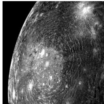
Figure 7.13: Valhalla, multi-ring impact basin on Callisto; the diameter of the ring system is ~3,800 km.
