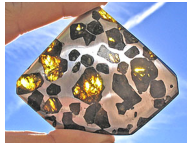
Figure 7.32: Slice of the Esquel pallasite, found in Argentina in 1951.
