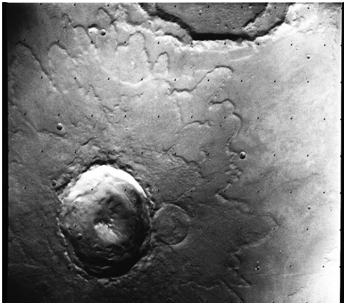
Figure 7.11: Yuty, Martian rampart crater, showing the lobate ejecta characteristic of rampart craters.
