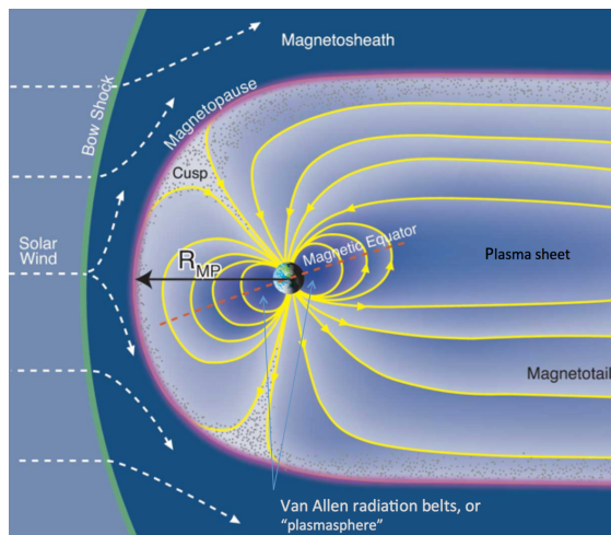
Figure 9.24: Earth's magnetosphere
