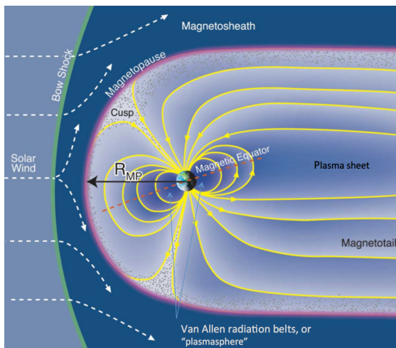
Figure 9.24: Earth's magnetosphere
