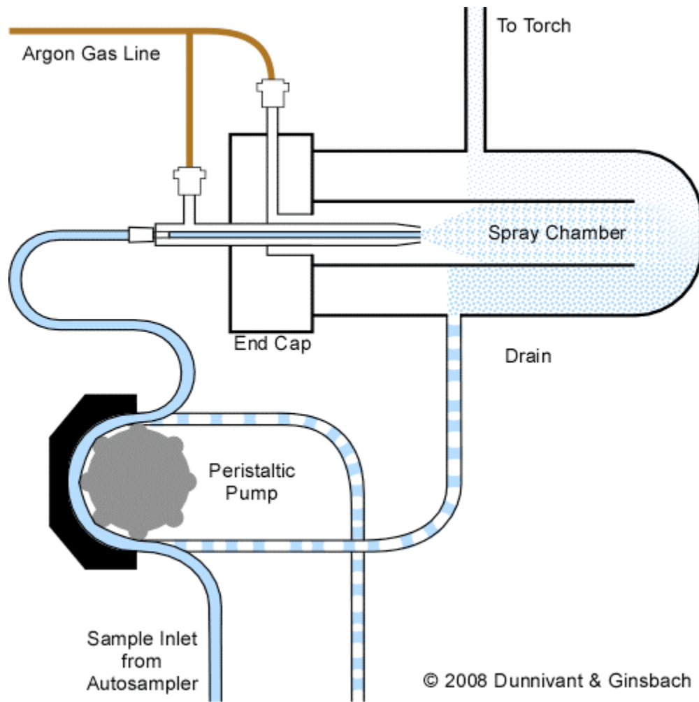
Figure 3-2. An Overview of Sample Introduction and the Nebulizer Chamber. (The nebulizer shown here is a pneumatic style, described below.)
