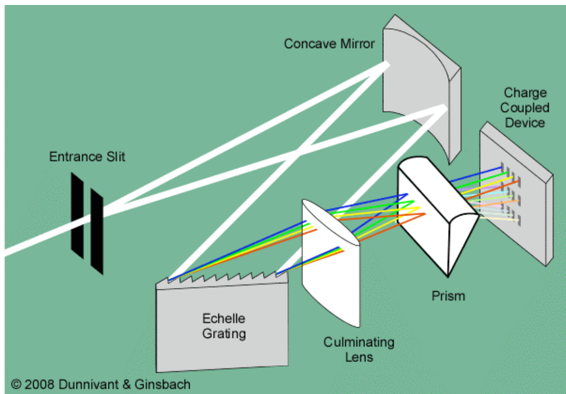
Figure 3-8. A Multiple Monochromator ICP-AES Instrument.
