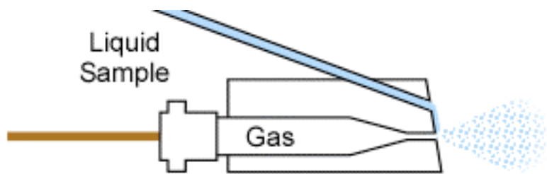
Figure 3-3. Diagram of a Pneumatic Concentric Nebulizer.
