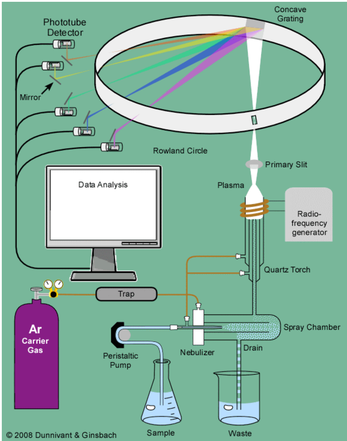
Figure 3-1. Overview of a Basic Inductively Coupled Plasma—Atomic Emission Spectrometry (ICP-AES) from the 1990s.
