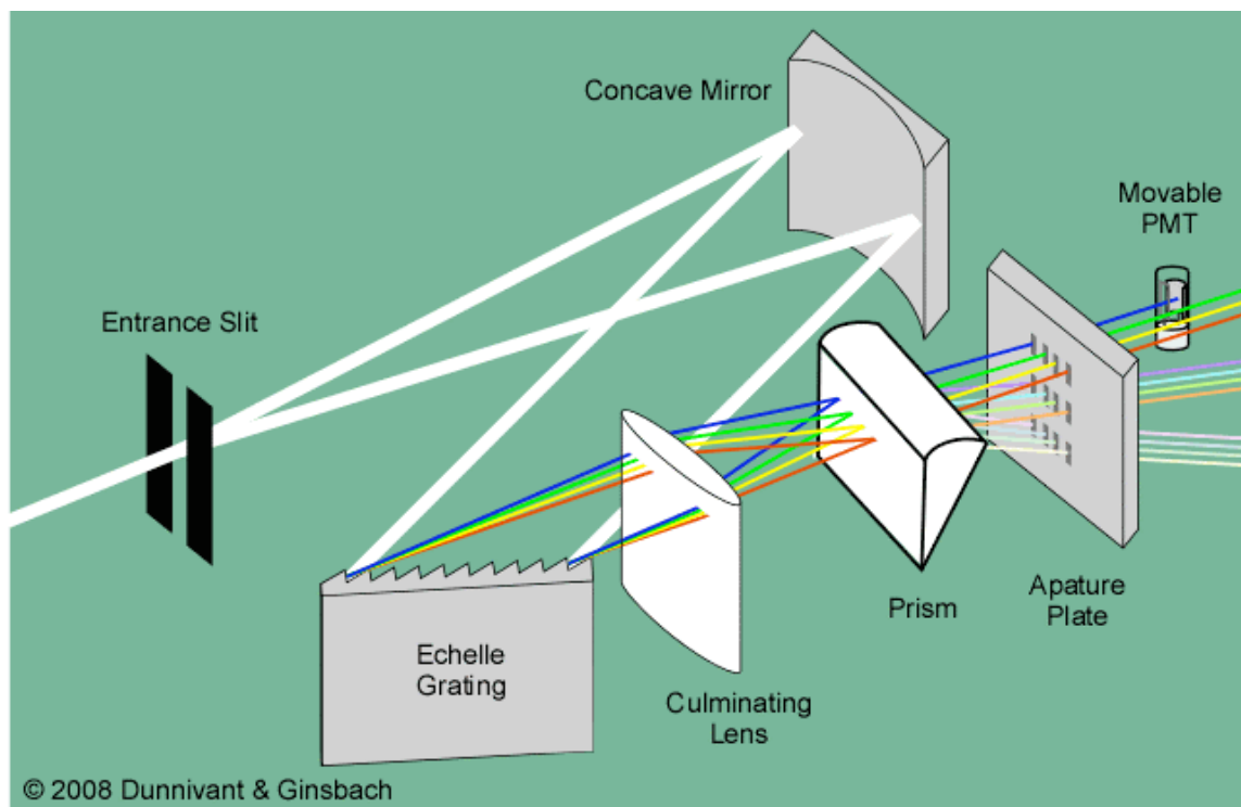
Figure 3-6. A Single Detector (sequential type monochromator) ICP-AES System.
