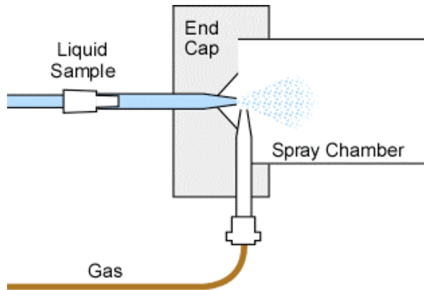
Figure 3-5. Diagram of a Pneumatic Cross-Flow Nebulizer.
