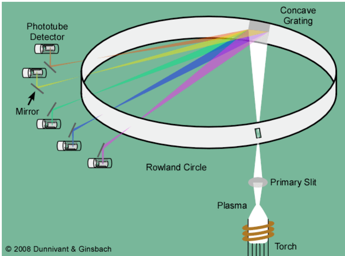
Figure 3-7. A Rowland Circle ICP-AES System.
