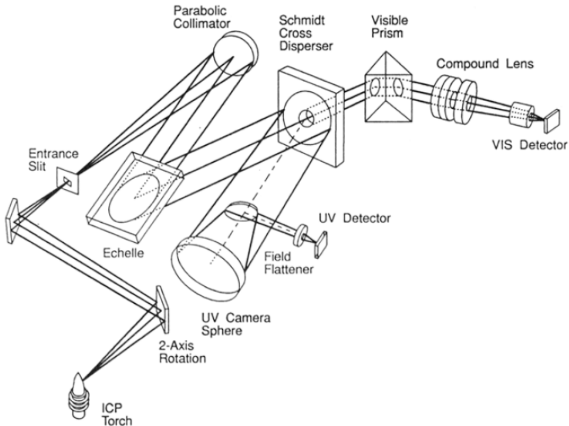
Figure 3-9. A Dual Echelle Grating – Prism Monochromator ICP with Dual CCD Detectors. From Barnard et al., Anal. Chem. , 1993, 65, 1231. Reprinted with permission from ACS.
