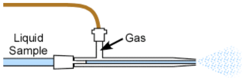
Figure 3-3. Diagram of a Pneumatic Concentric Nebulizer.
