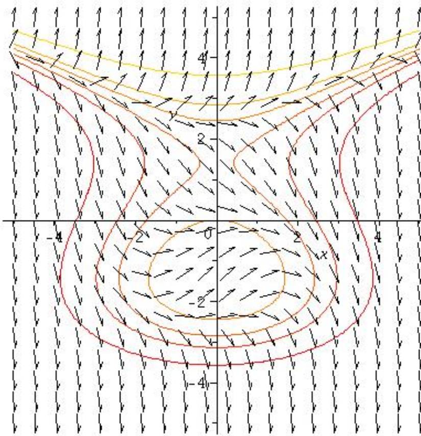
Figure 1: Isoclines as contours of \frac{1}{6}y^3 - y - \frac{1}{3}t^2 , and the isoclines superimposed on the direction field. Can you tell which contours I plotted?
