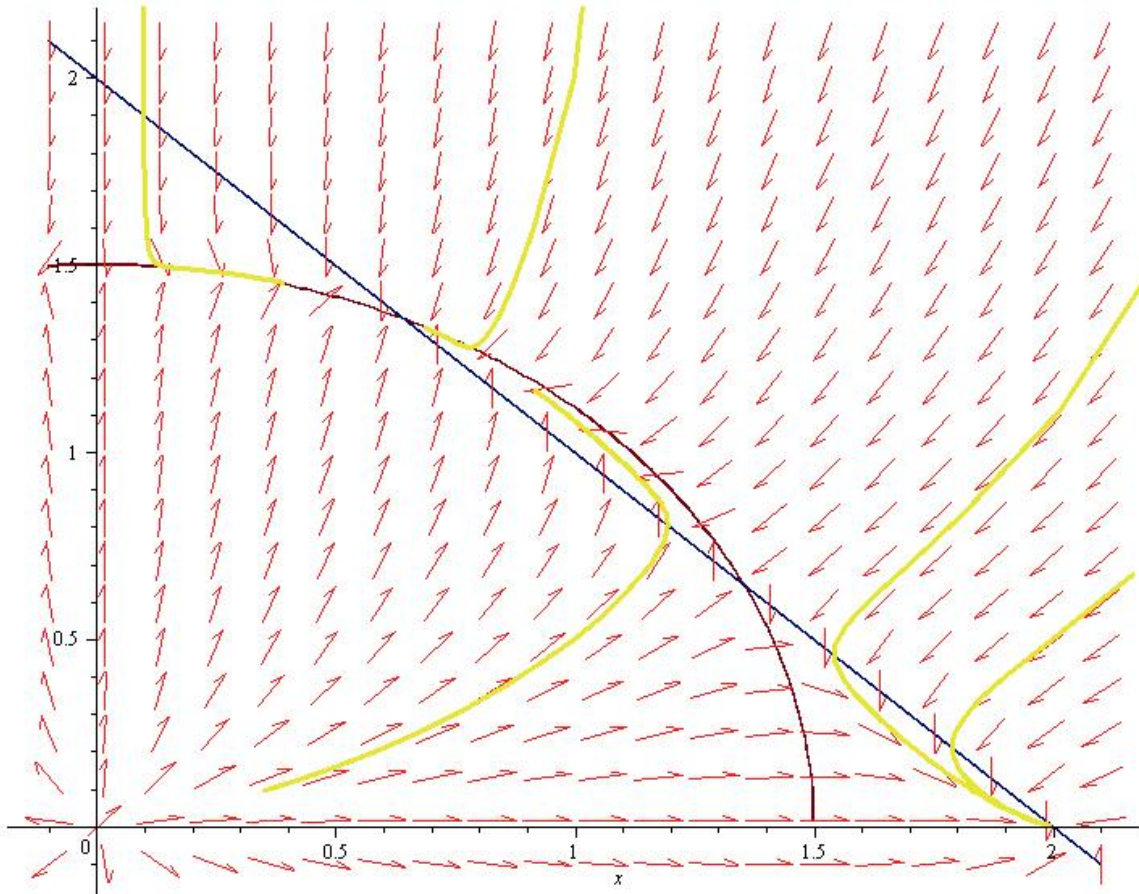
Figure 1: Nullclines and some solutions to x' = x(2 - x - y) , y' = y(9/4 - y^2 - x^2)
