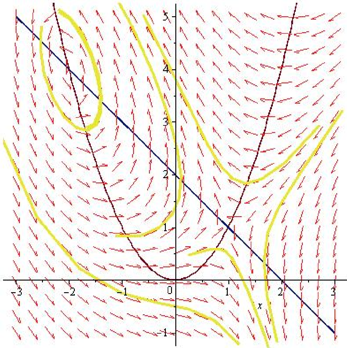
Figure 3: Nullclines and some solutions to x' = 2 - x - y , y' = y - x^2
