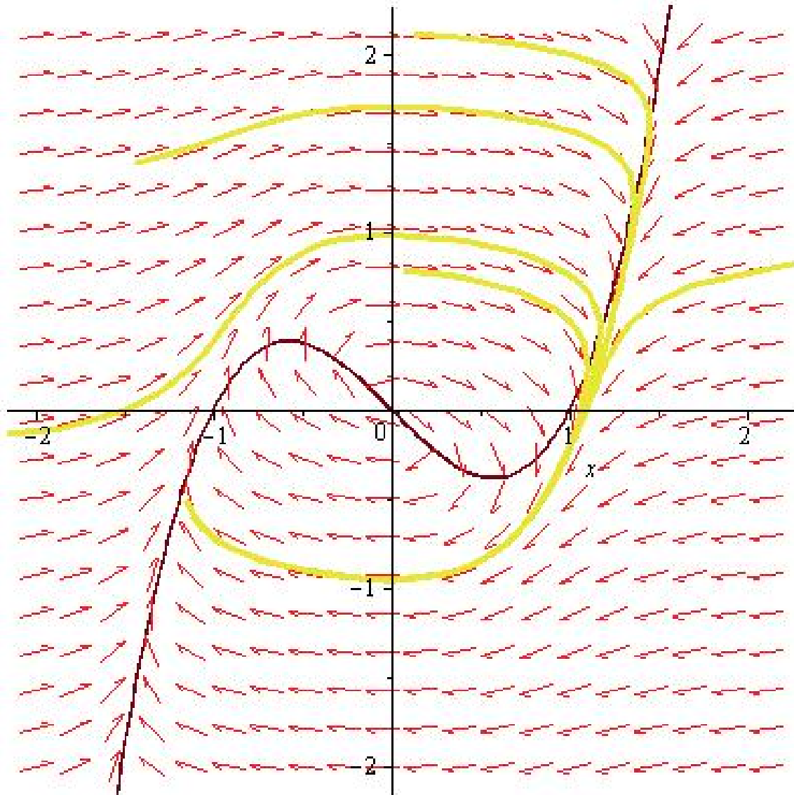
Figure 2: Nullclines and some solutions to x' = x + y - x^3 , y' = -\frac{1}{2}x
